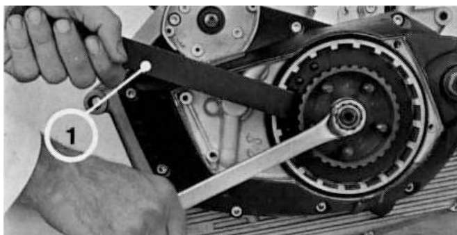
1. Clutch holder - special tool 001 - attrezzo speciale 001
